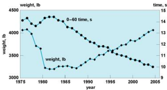
Fig. 1 Change in vehicle weight and acceleration performance from 1975 to 2004 ( U.S. EPA Light-Duty Automotive and Fuel Economy Trends: 1975–2004, April 2004 ).
